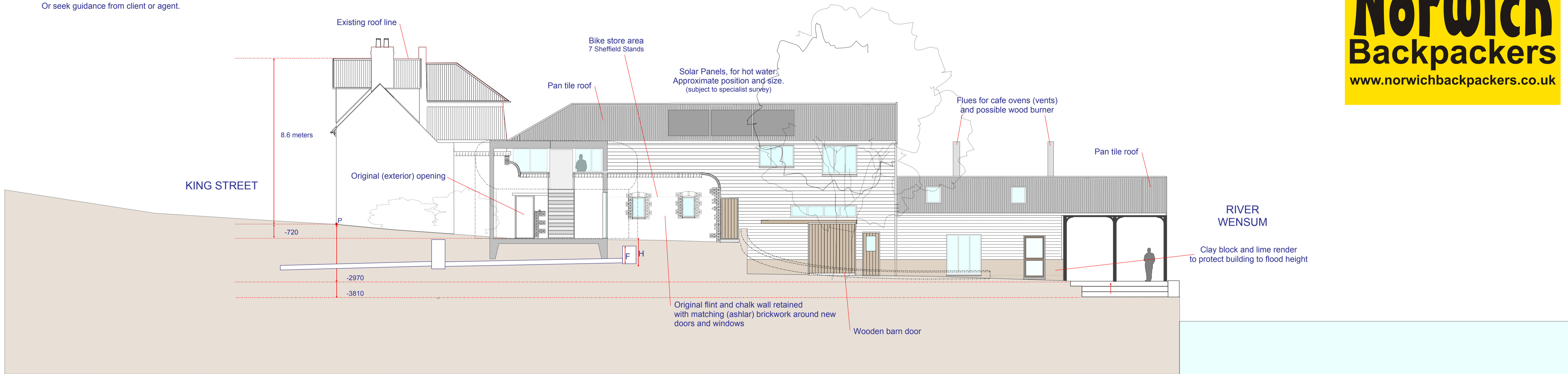
Norwich Backpackers from the SOUTH SIDE, point A, with RECEPTION section. PROPOSED
