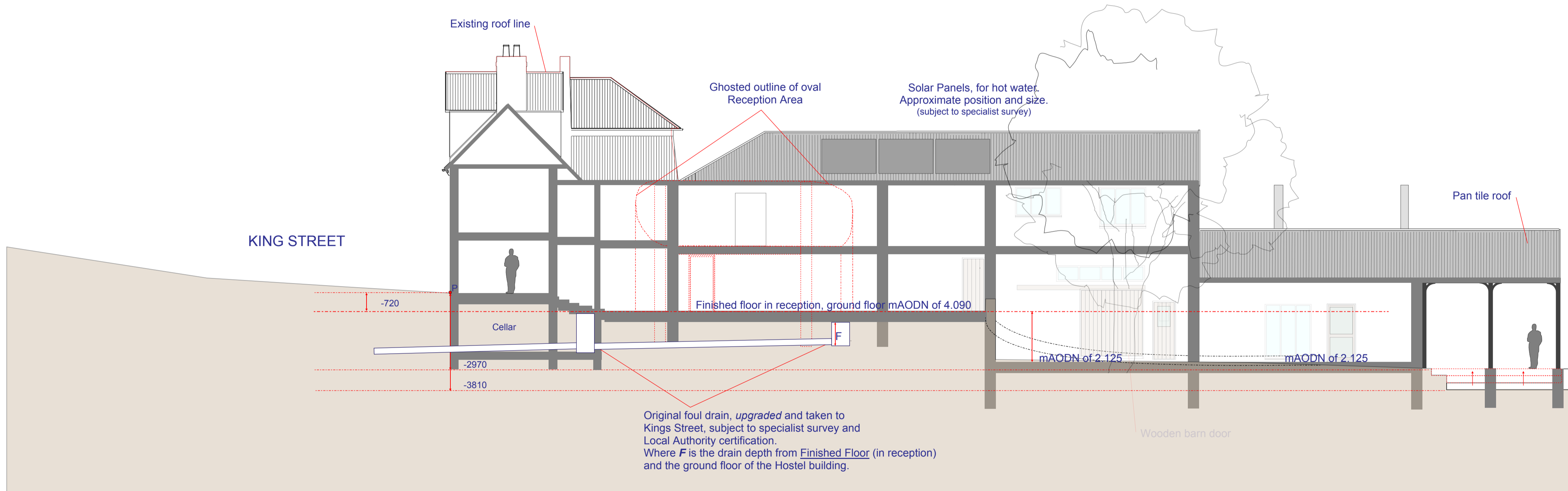
Norwich Backpackers from the SOUTH SIDE showing SECTION with basic structure.
