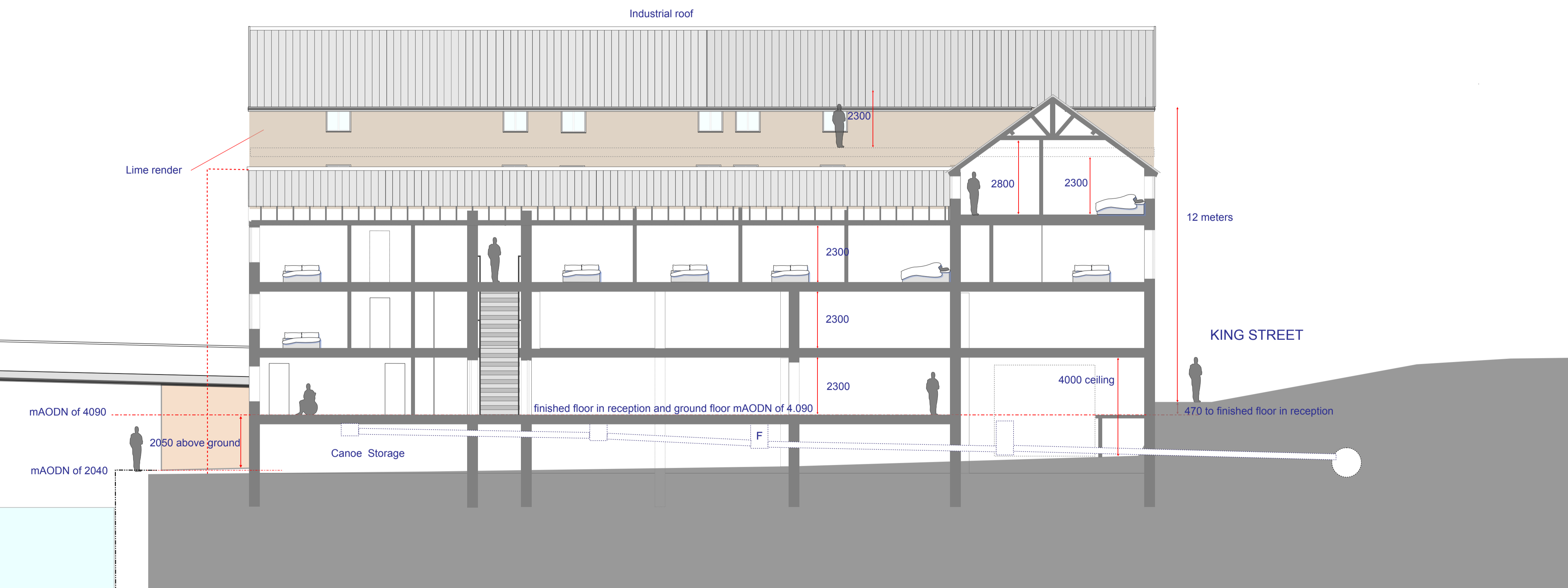
The FERRY BOAT SECTION from G, CAR PARK to BRIDGE, proposed
